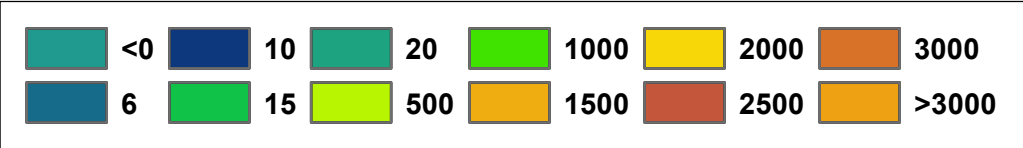
2005 Reclassified DEM of Gulf Coast (meters)
